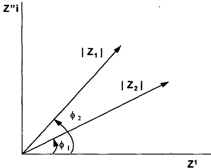
Figura1.1. Diagrama de Argand.
