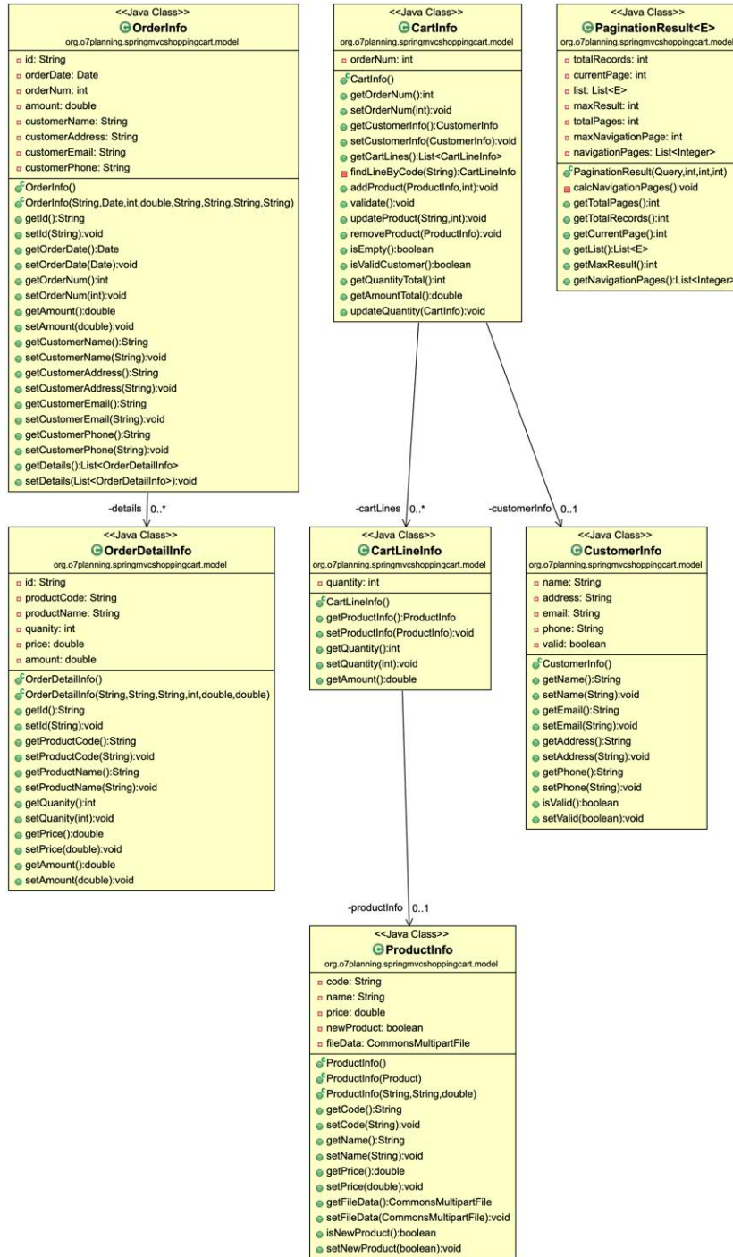
Figura A.7: UML de org.o7planning.springmvcshoppingcart.model
