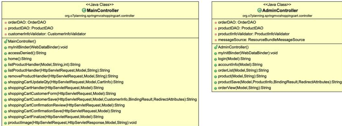
Figura A.4: UML de org.o7planning.springmvcshoppingcart.controller
