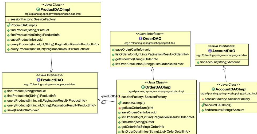
Figura A.5: UML de org.o7planning.springmvcshoppingcart.dao y dao.impl
