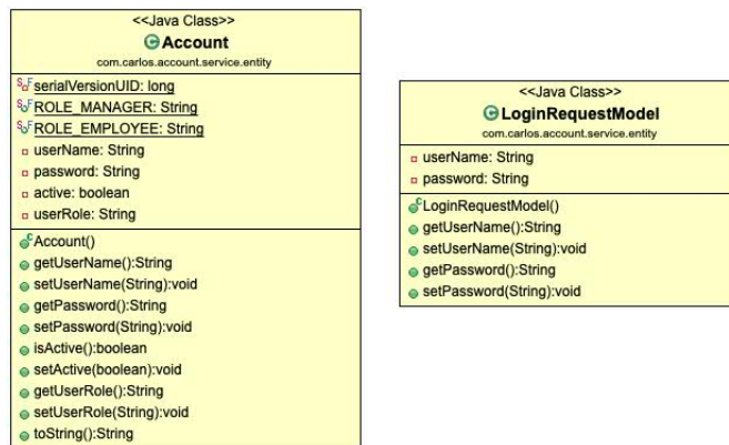
Figura B.5: UML de com.carlos.account.service.entity
