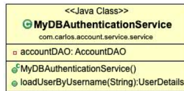
Figura B.2: UML de com.carlos.account.service.service
