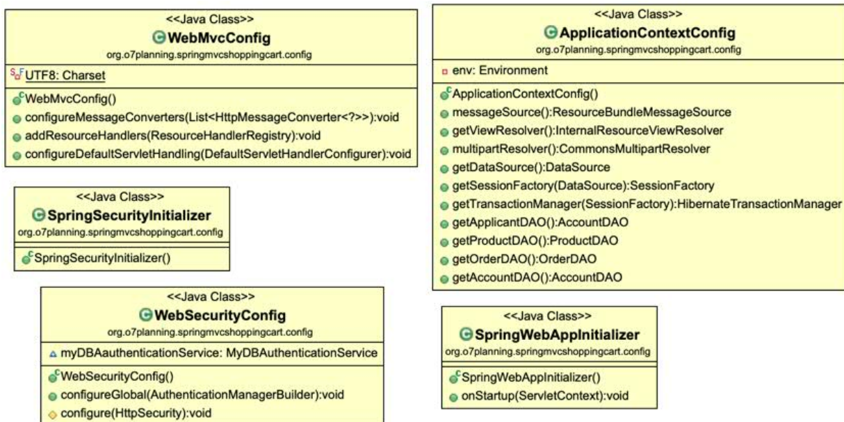
Figura A.3: UML de org.o7planning.springmvcshoppingcart.config
