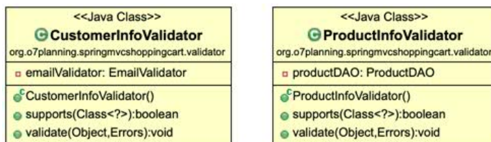
Figura A.9: UML de org.o7planning.springmvcshoppingcart.validator
