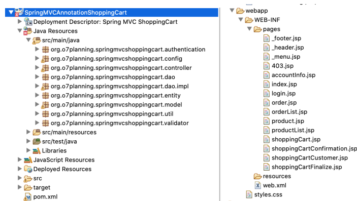
(a) Paquetes Java
