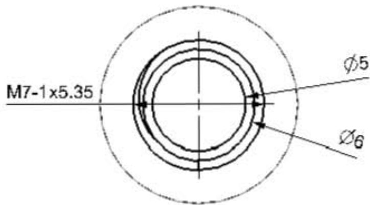
DETAIL A SCALE 5:1
