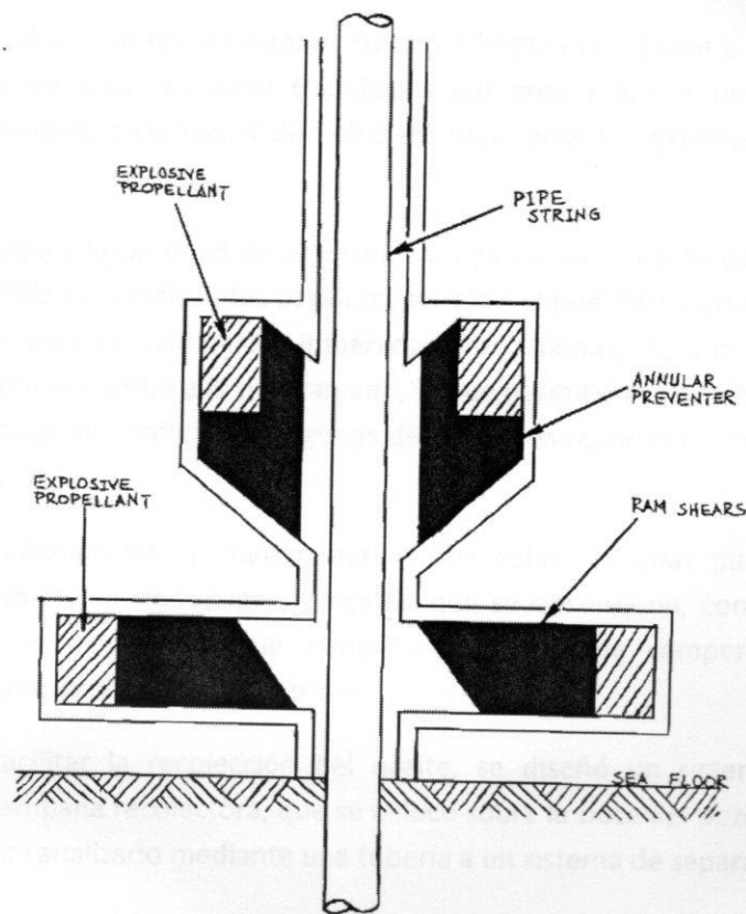
Figure 4: Blowout Preventer (Schematic)
