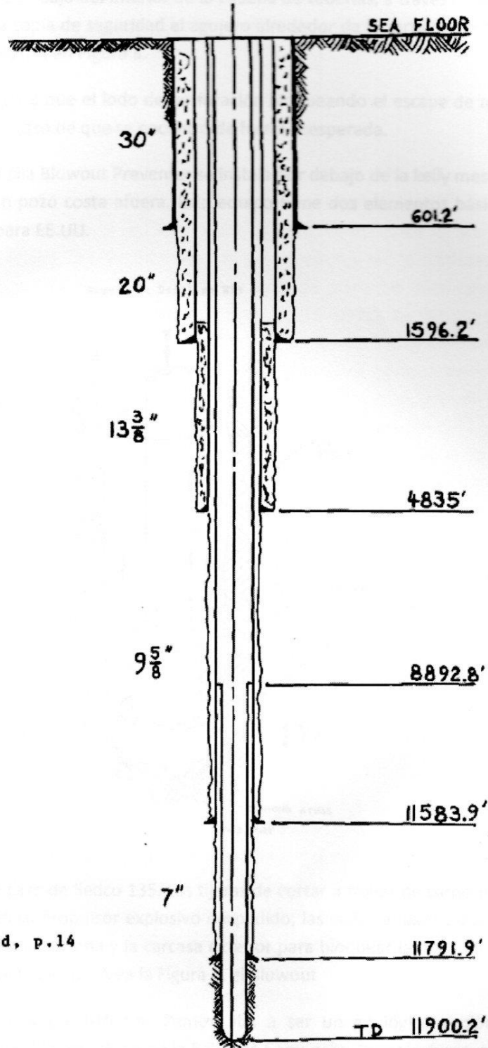
Figure 2: IXTOC I Casing Strings
