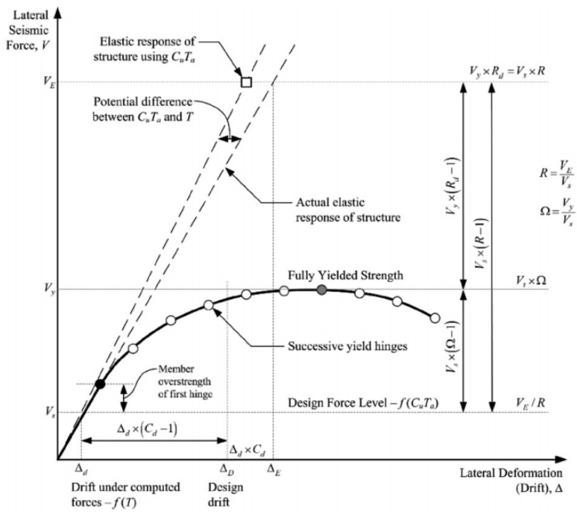
Figure 3: System parameter definitions from a pushover curve.
