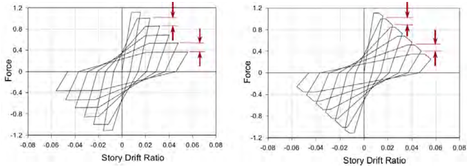
Figure 8: Cyclic and in-cycle strength degradation [FEMA, 2009]
