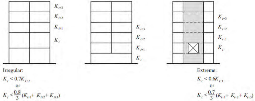
Figure 2: Conditions for soft or extreme soft-storey according to ASCE7
