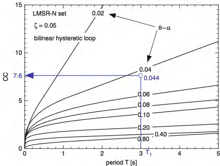
Figure 11: Application of a collapse-capacity spectra to an equivalent non-deteriorating sdf [Adam and Jäger, 2012a]
