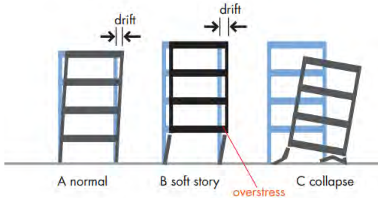
Figure 5: Sidesway-collapse of a soft-first-storey building
