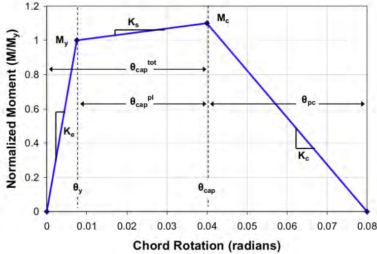
Figure 9: Hysteretic backbone curve according to the IMK model for reinforced concrete
