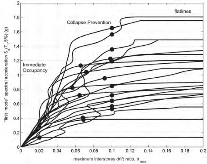
Figure 10: Example of IDA curves for a set of records, showing the flattening portion of the curve indicative of dynamic instability [Vamvatsikos, 2004]
