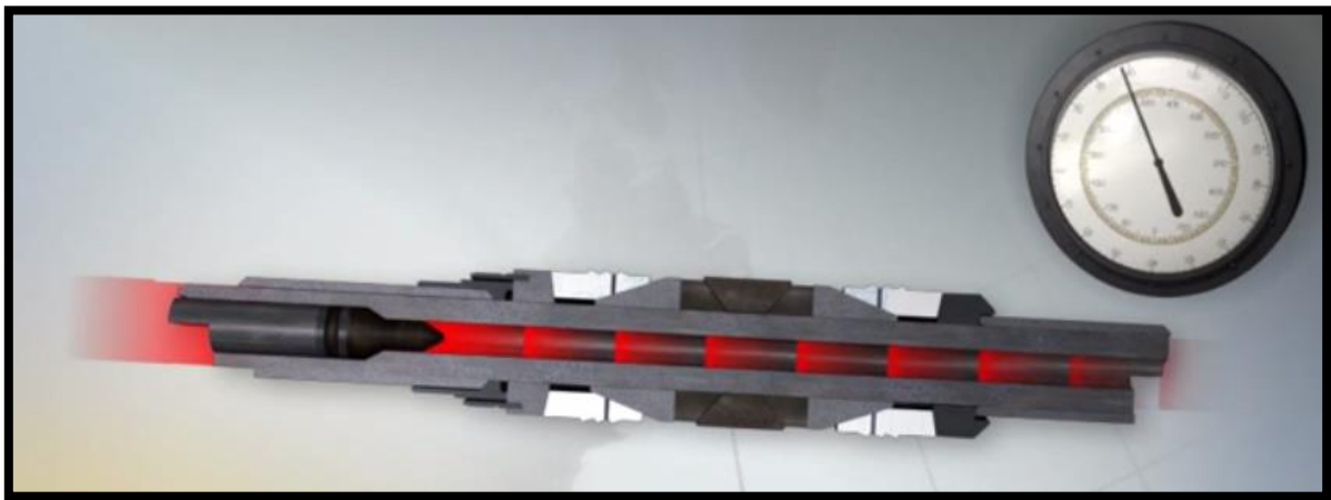
Figura 4.3. Bridge plug. Recuperado de [ http://www.youtube.com/watch?v=oPgZnZqp87k ]
