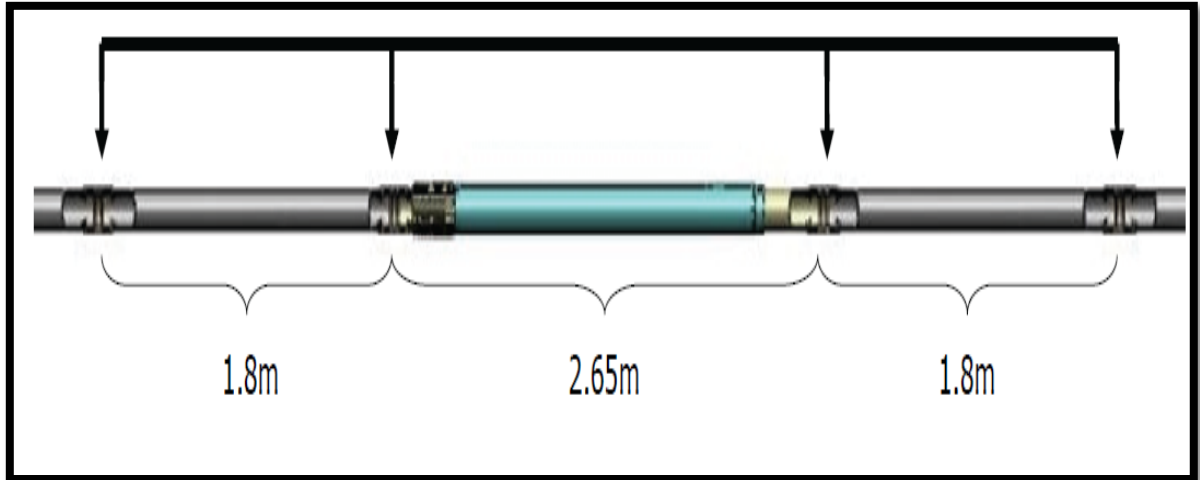
Figura 4.17. Collar localizador Mecánico. Recuperado de [Cased-Hole Multistage Fracturing: A new Coiled-tubing-enable completion. Ravensberg J. & baker hughs. (2011).]
