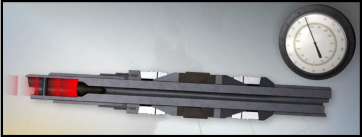
Figura 4.4. Proppet style frac plug. Recuperado de [http://www.youtube.com/watch?v=oPgZnZqp87k]
