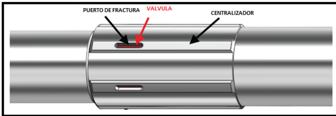
Figura 4.11. Camisa Hidraulica Fracport. Recuperado de [Cased-Hole Multistage Fracturing: A new Coiled-tubing-enable completion. Ravensberg J. & baker hughs. (2011).]
