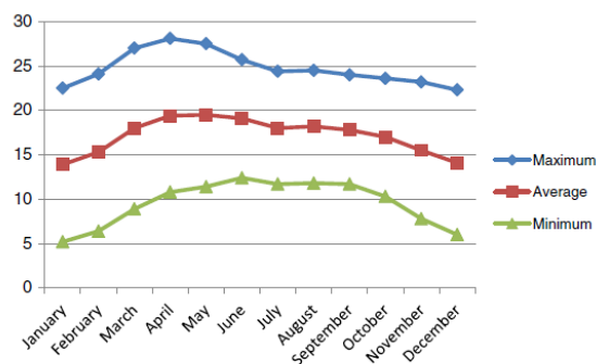
Fig. 2. Monthly average temperature over 30 years in Santa Úrsula Coapa, Mexico City (°C).
