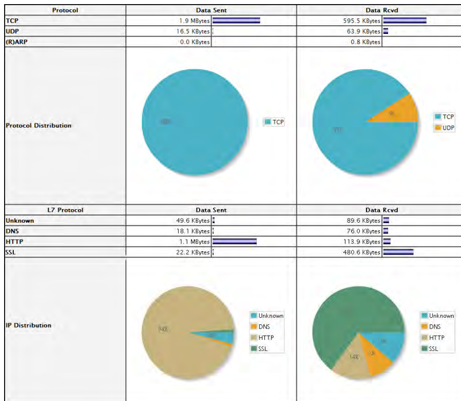
Figura 5.8: Ntop - Protocolos
