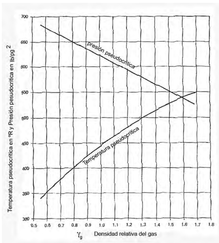
Figura 1.3 Propiedades pseudocríticas de los gases naturales. (R.P. Sutton "Compressibility Factors for High-Molecular-Weight Reservoir Gases" Paper SPE 14265)
