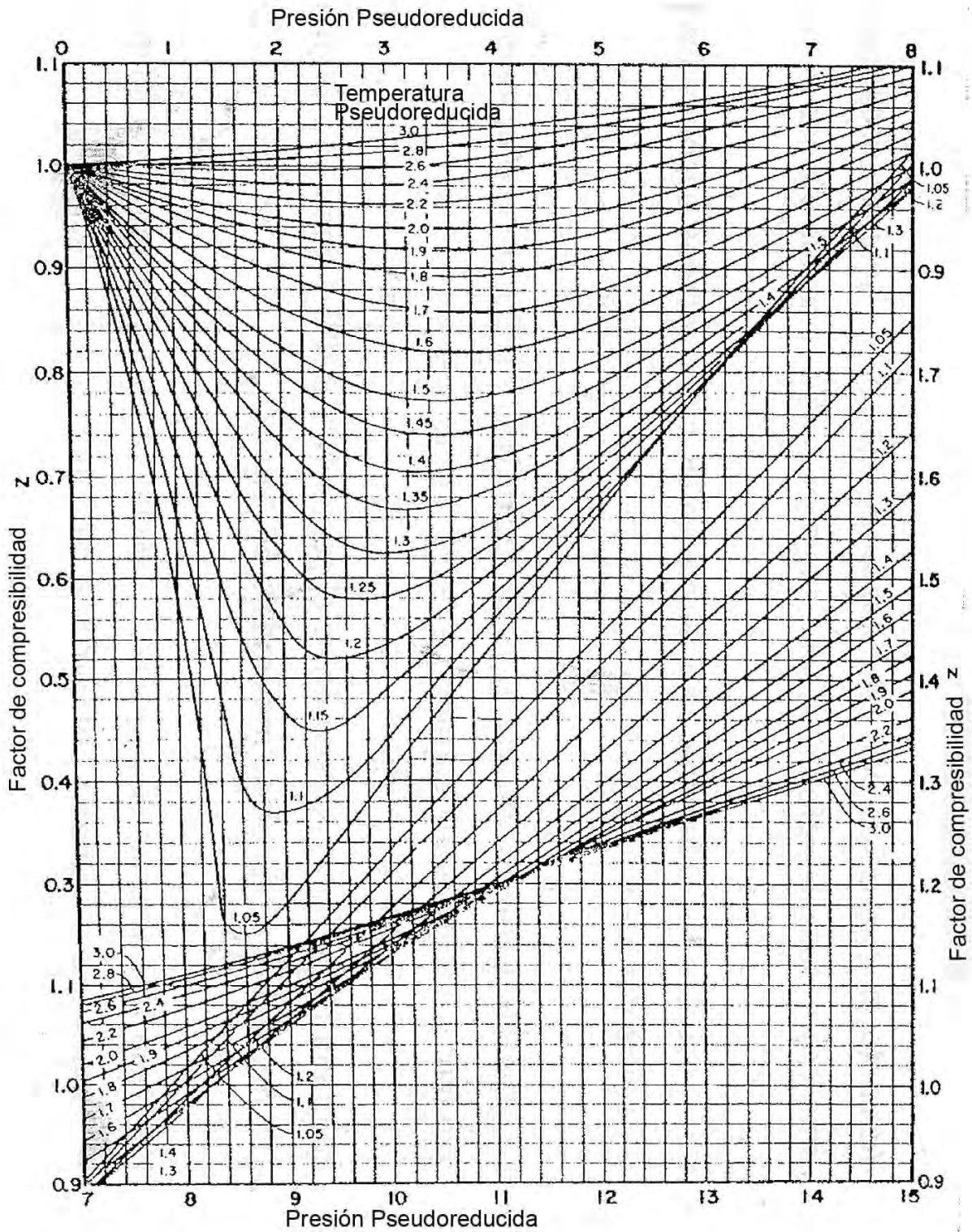
Figura 1.4 Factores de compresibilidad para gases naturales (Standing and Katz, Trans, AIME, 146,140, Copyright 1942 SPE-AIME)
