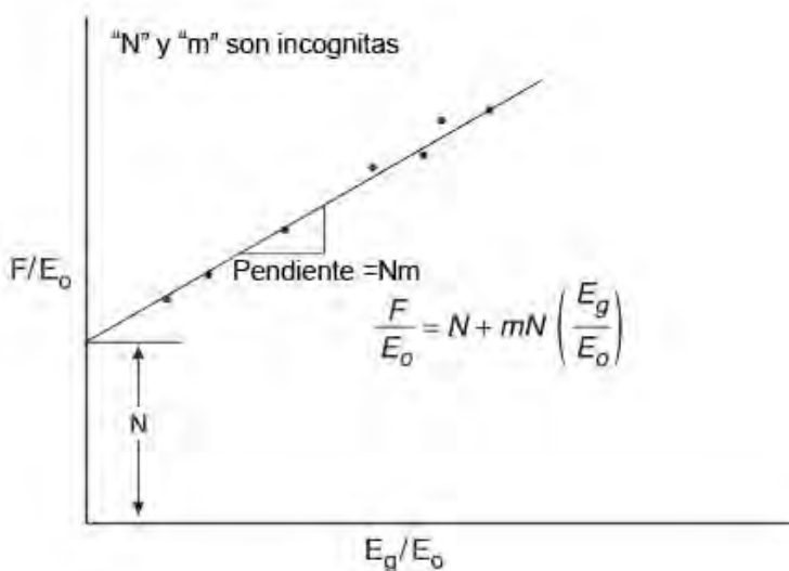
Figura 4.18 F/E_o vs. E_g/E_o .
