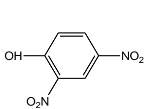
Dinitrofenol (DNP)
