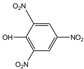
trinitrofenol(TNP)
