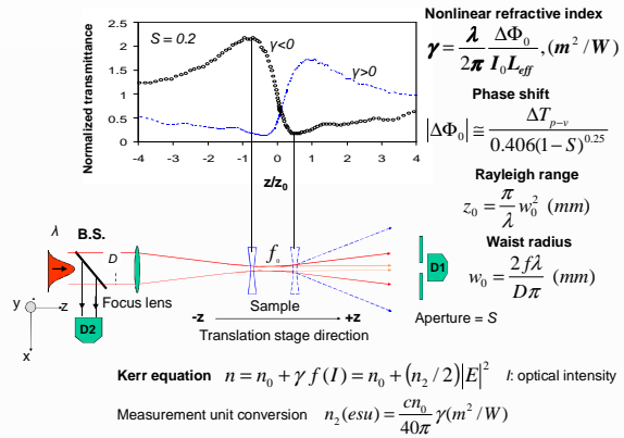
Figure 1. Variation of IDRI \gamma , due of the Kerr-based effect as a function of intensity I and diameter of aperture S .
