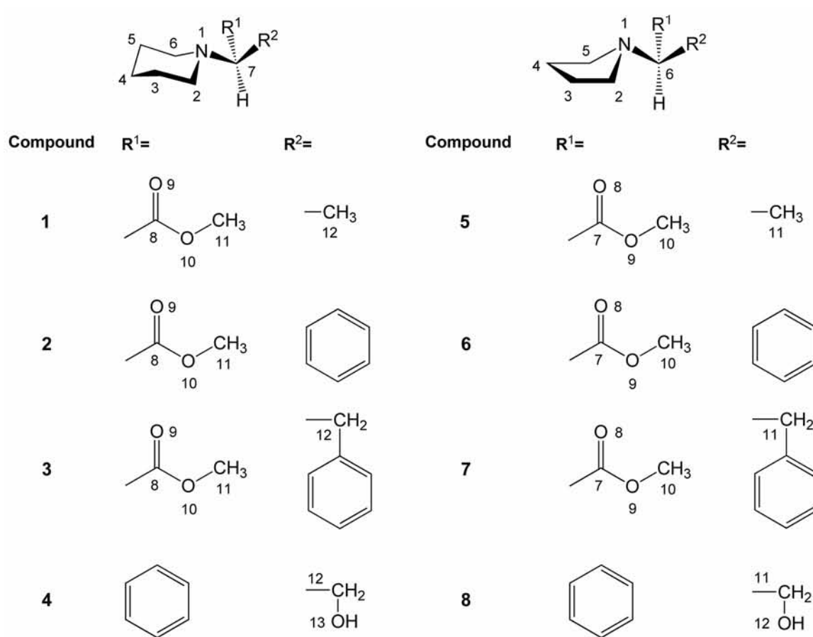
Fig. 2. Numbering System for Structures 1-8.
