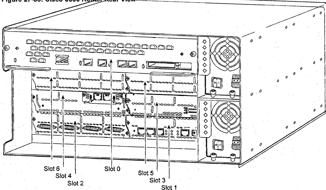
Figure 27-35: Cisco 3660 Router Rear View
