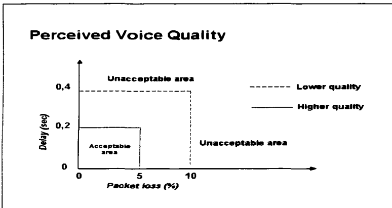
Figura III.38.- Perceived Voice Quality.
