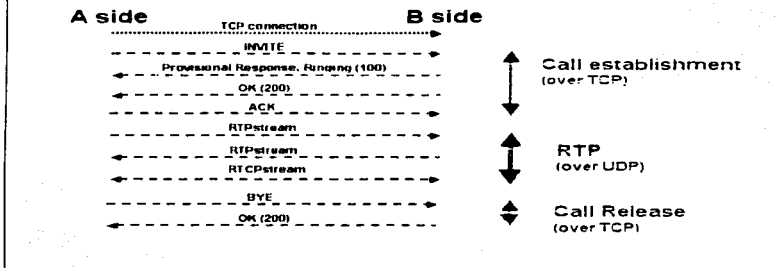
Figura III.56.- SIP Call Setup.
