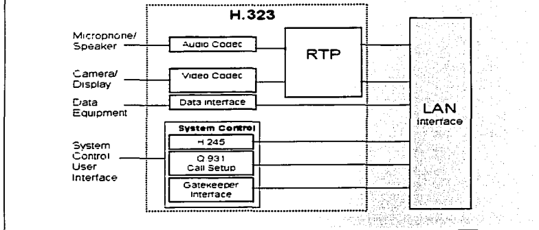
Figura III.18.- H.323 Funtional Structure.
