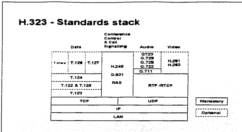
Figura III.19.- H.323 Standards Stack.
