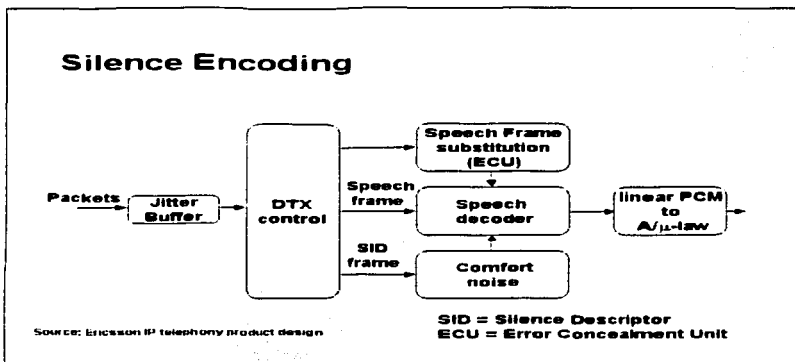
Figura III.39.- Silence Encoding.
