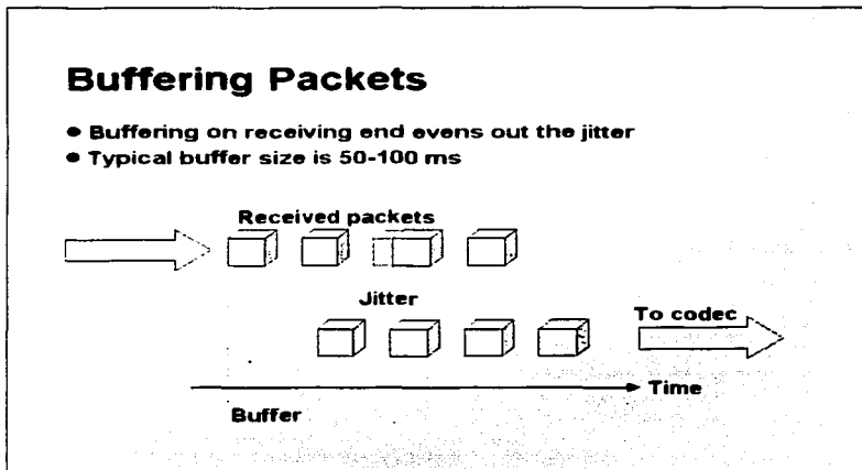
Figura III.36.- Buffering Packets.
