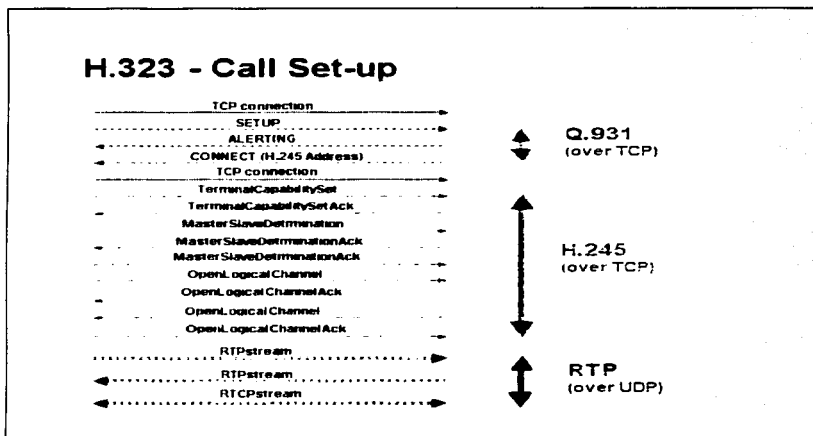
Figura III.24.- H.323 – Call-set-up.
