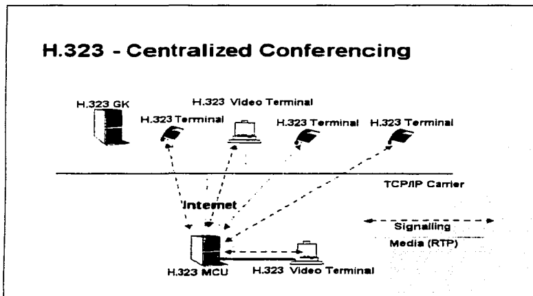
Figura III.27.- H.323 – Centralizad Conferencing.
