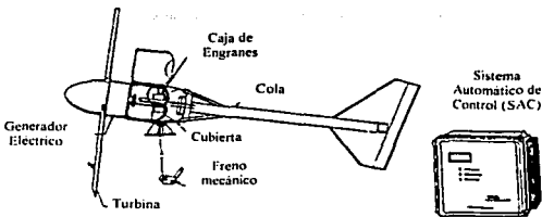
Figura 3.20: Aerogenerador de eje horizontal de 10 kW. BWC Excel-R Owner's Manual and Part List.
