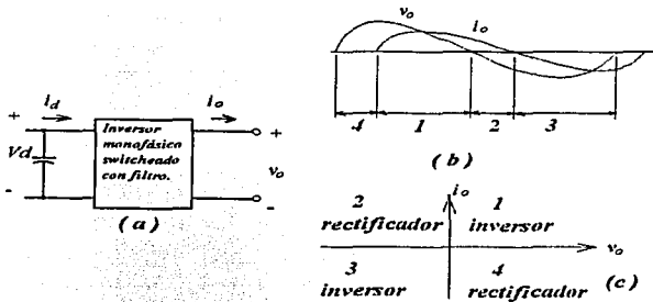
Figura 6.5. Inversor monofásico conmutado. (Power Electronics: Converters, Applications and Design).
