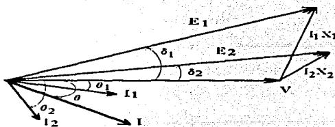
Figura 6.21. Diagrama fasorial del sistema. (Novel Wind/Diesel/Battery Hybrid Energy System).
