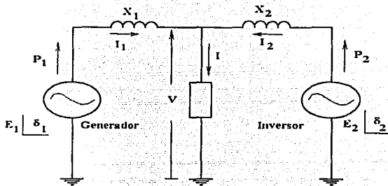
Figura 6.20. Circuito equivalente del sistema. (Novel Wind/Diesel/Battery Hybrid Energy System).
