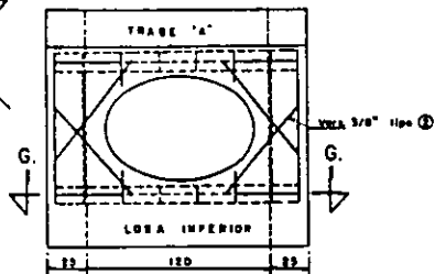
LOSA LATERAL
