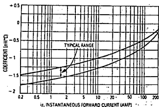
Figure 3. Forward Voltage Temperature Coefficient
