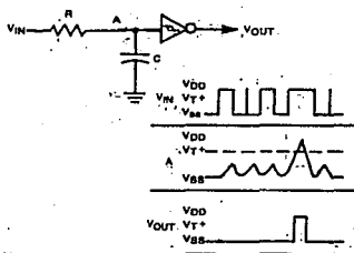
FIGURE 6 — INTEGRATOR
