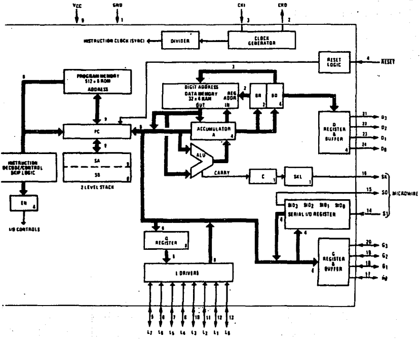
Fig. III.2.2.4 Diagrama a bloques del MCU COP4101.
