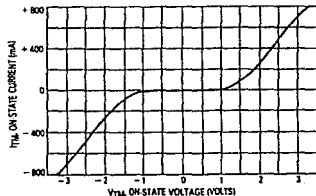
Figure 2. On-State Characteristics
