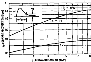
Figure 8. Forward Recovery Time
