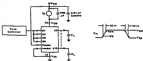
FIGURE 3 - DYNAMIC POWER DISSIPATION TEST CIRCUIT AND WAVEFORM
