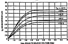
FIGURE 4 - V_{GS} = 10 \text{ Vdc}
