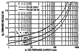
Figure 1. LED Forward Voltage versus Current
