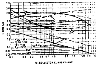
FIGURE 3 - SWITCHING TIMES
