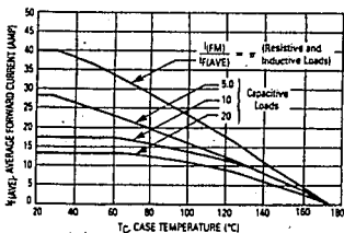
Figure 4. Current Derating
