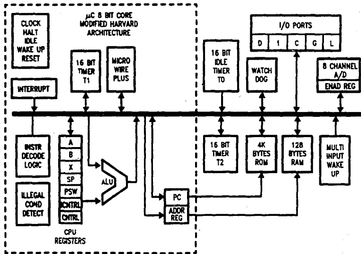
Fig. III.2.2.11 Diagrama a bloques del MCU COP888CF.
