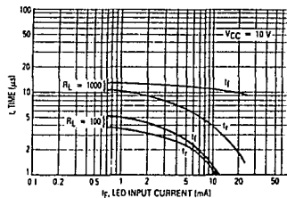
Figure 6. Rise and Fall Times
