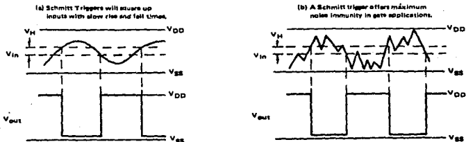
FIGURE 2 - TYPICAL SCHMITT TRIGGER APPLICATIONS
