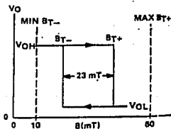
FIGURE 2. REPRESENTATIVE CURVE OF V_{O} VS B
