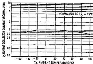
Figure 4. Output Current versus Ambient Temperature
