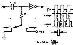
FIGURE 7 — DIFFERENTIATOR
