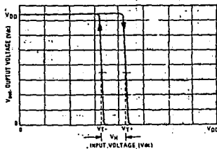
FIGURE 2 — TYPICAL TRANSFER CHARACTERISTICS
