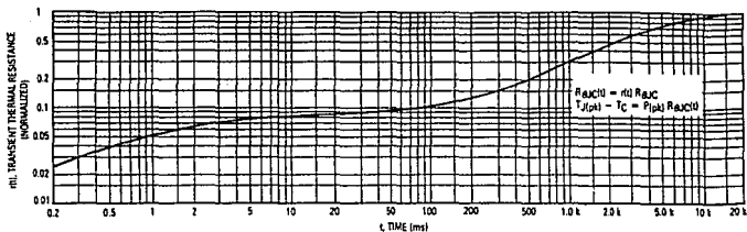
Figure 6. Typical Thermal Response
