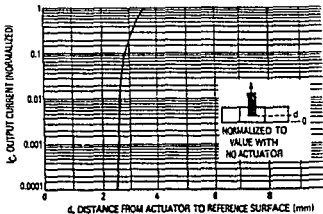
Figure 2. Output Current versus Actuator Reference
