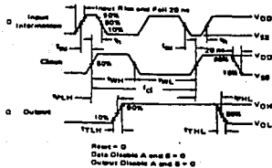
FIGURE 1 - TIMING DIAGRAM
