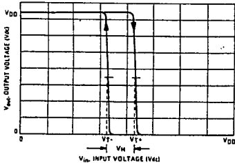
FIGURE 5 - TYPICAL TRANSFER CHARACTERISTICS
