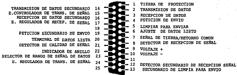
Fig. II.5a.2 Interface RS232C.
