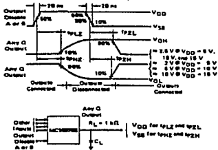
FIGURE 2 - THREE-STATE PROPAGATION DELAY WAVEFORM AND CIRCUIT
