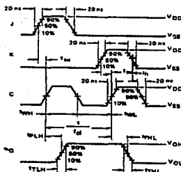
FIGURE 1 — DYNAMIC SIGNAL WAVEFORMS (J, K, Clock, and Output)
