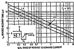
Figure 9. Reverse Recovery Time
