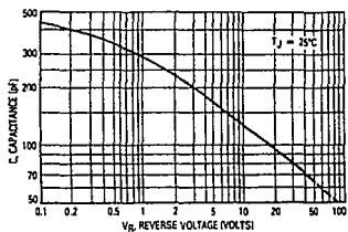
Figure 7. Capacitance
