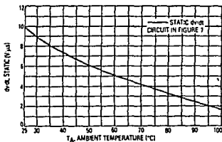
Figure 5. dV/dt versus Temperature
