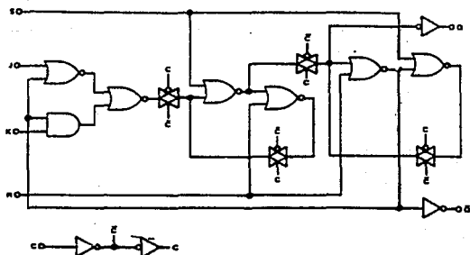
LOGIC DIAGRAM (1/2 of Device Element)
