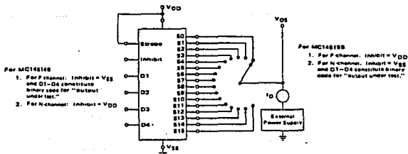
FIGURE 1 — DRAIN CHARACTERISTICS TEST CIRCUIT
