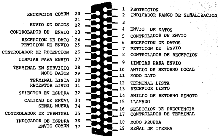
Fig. II.5b.4 Interface RS422. II - 190
