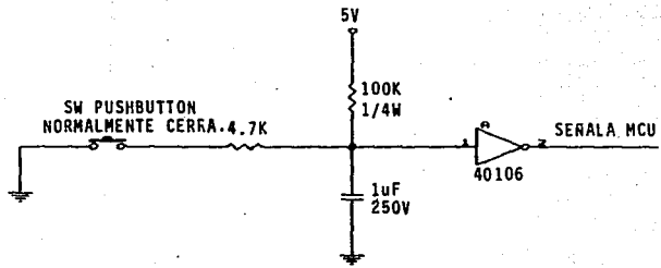
Fig. III.3a.7 Circuito interruptor de reset. III - 101
