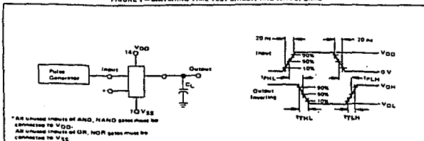
FIGURE 1 — SWITCHING TIME TEST CIRCUIT AND WAVEFORMS
