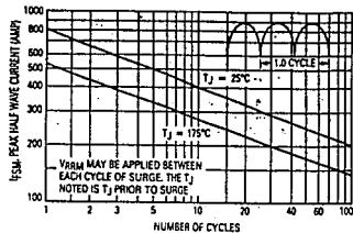
Figure 2. Non-Repetitive Surge Current
