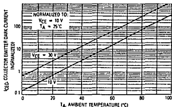
Figure 5. Dark Current versus Ambient Temperature
