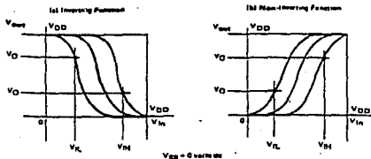
FIGURE 11 - DC NOISE IMMUNITY
