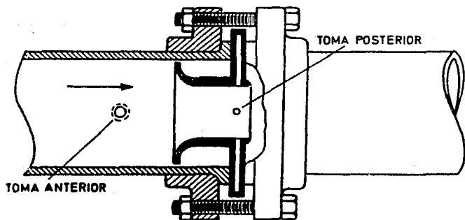
Fig. II.1.2.10 Tobera.
