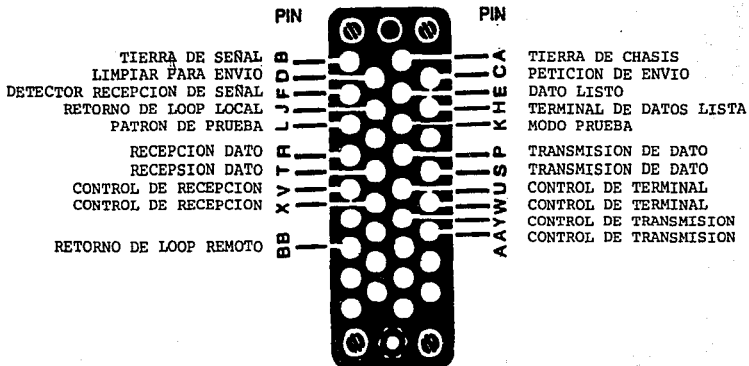
Fig. II.5c.4 Interface RS485.
