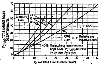
Figure 5. Forward Power Dissipation
