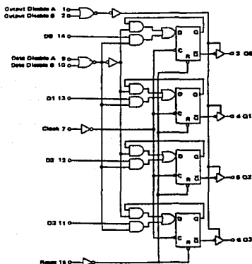
EQUIVALENT FUNCTIONAL BLOCK DIAGRAM
