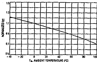
Figure 3. Trigger Current versus Temperature
