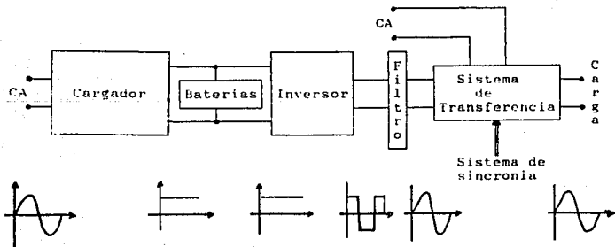
Fig. III.3d.2 Diagrama a bloques del UPS Off-Line.
