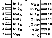
PIN ASSIGNMENT
