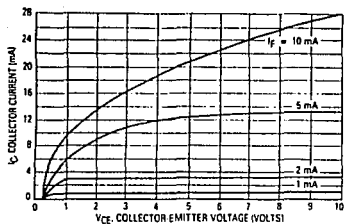
Figure 3. Collector Current versus Collector-Emitter Voltage
