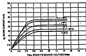
FIGURE 6 - V_{GS} = 18 \text{ Vdc}
