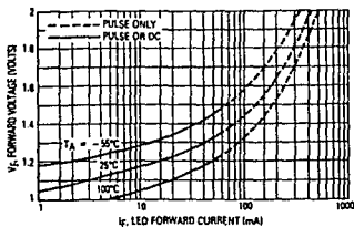
Figure 1. LED Forward Voltage versus Forward Current
