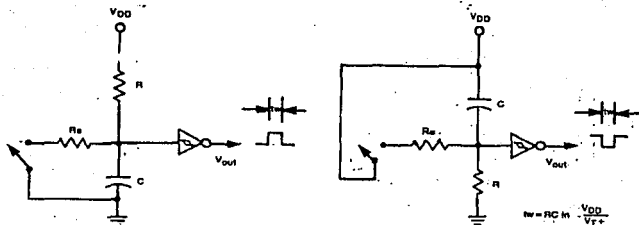
FIGURE 4 — MONOSTABLE MULTIVIBRATOR
