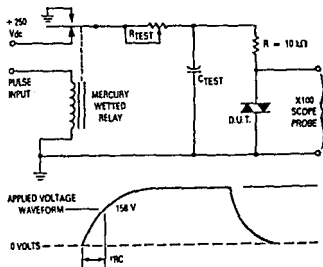
Figure 7. Static dV/dt Test Circuit
