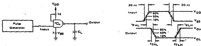
FIGURE 1 - SWITCHING TIME TEST CIRCUIT AND WAVE FORMS
