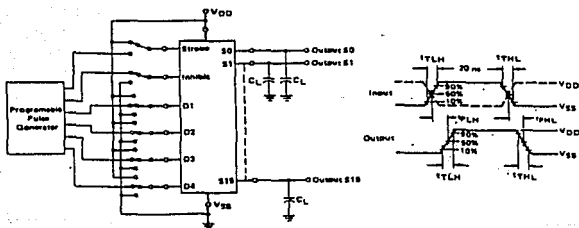
FIGURE 3 - SWITCHING TIME TEST CIRCUIT AND WAVEFORMS
