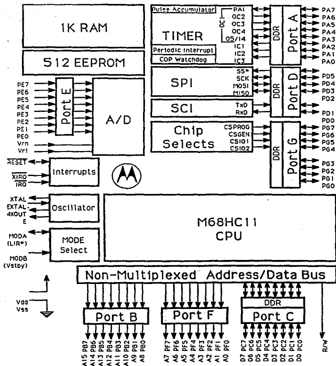
Fig. III.2.3.3 Diagrama a bloques del MCU 68HC11F1.
