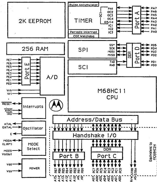
Fig. III.2.3.4 Diagrama a bloques del MCU 68HC11E2.
