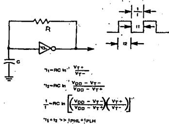
FIGURE 5 — ASTABLE MULTIVIBRATOR
