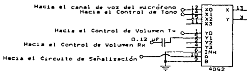
Diagrama 6. Multiplexor 1/Demultiplexor 1.
