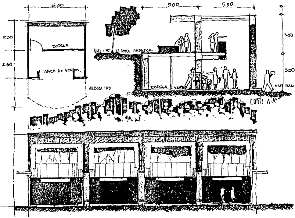
FACHADA PRINCIPAL
