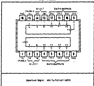
SN54LS139, SN54S139 . . . J OR N PACKAGE SN74LS139, SN74S139 . . . J OR N PACKAGE (TOP VIEW)
