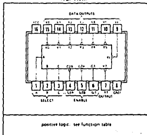
SN54LS138, SN54S138 . . . J OR N PACKAGE SN74LS138, SN74S138 . . . J OR N PACKAGE (TOP VIEW)
