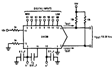
FIGURE 1. \pm 20 V pp Output Digital-to-Analog Converter
