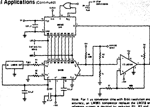
FIGURE 27. A Complete 2 \mu\text{s} Conversion Time, 8-Bit A/D Converter
