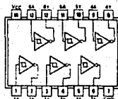
SN5414 (J, W) SN54LS14 (J, W)
