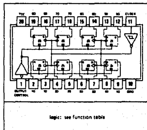
SN54LS374, SN54S374 ... J PACKAGE SN74LS374, SN74S374 ... J OR N PACKAGE (TOP VIEW)
