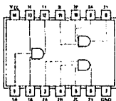
SN54H11 (J) SN54LS11 (J, W) SN54S11 (J, W)
