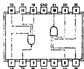
SN54H22 (W)
