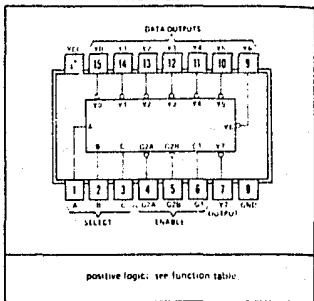
SN54LS138, SN54S138 ... J OR W PACKAGE SN74LS138, SN74S138 ... J OR N PACKAGE (TOP VIEW)
