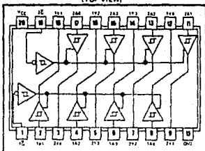
SN54LS244 ... J SN74LS244 ... J OR N (TOP VIEW)
