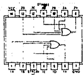
SN5425 (J, W) SN7425 (J, N)
