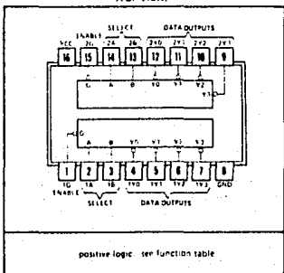
SN54LS139, SN54S139 ... J OR W PACKAGE SN74LS139, SN74S139 ... J OR N PACKAGE (TOP VIEW)
