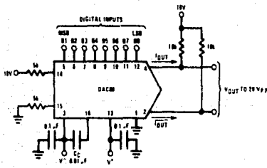
FIGURE 1. \pm 20 V p-p Output Digital-to-Analog Converter
