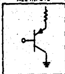
TYPICAL OF ALL INPUTS
