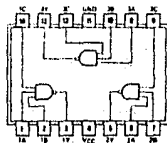
SN5410 (W) SN54H10 (W) SN54L10 (T)
