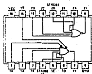
SN5423 (J, W) SN7423 (J, N)
