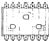
SN54H11 (W)
