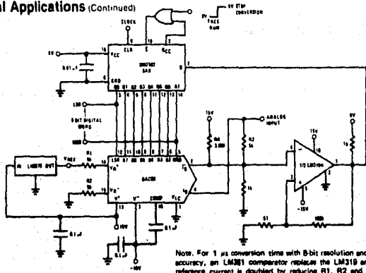
FIGURE 27. A Complete 2 μs Conversion Time, 8-Bit A/D Converter
