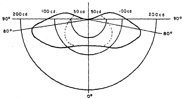
c) NON CUT-OFF (HAZ NO RECORTADO)
