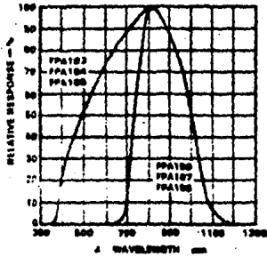
Spectral Characteristics
