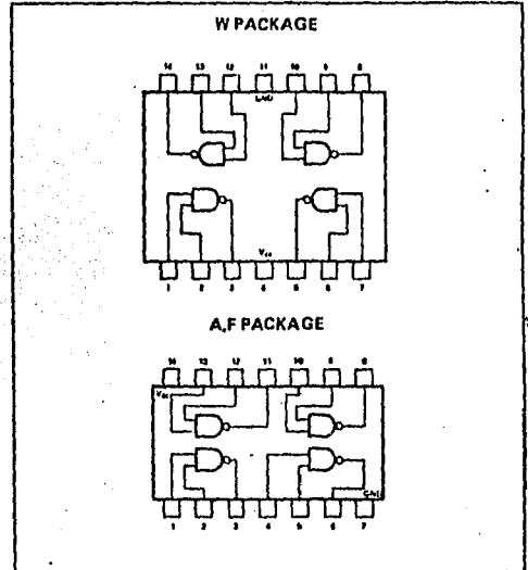
PIN CONFIGURATIONS
