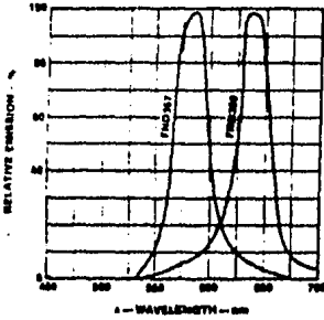
Emission Spectrum
