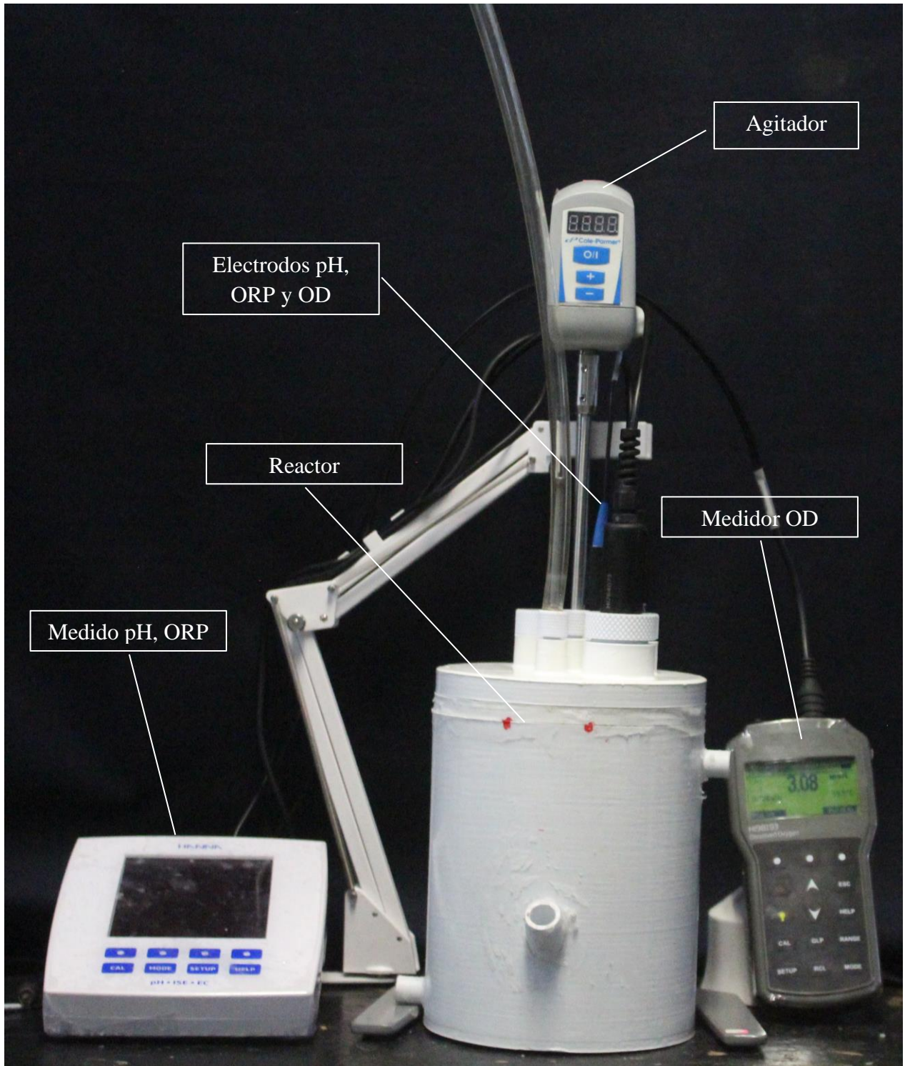
Figura 4 Reactor experimental.
