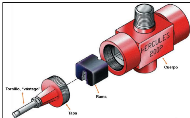
Figura 2.35 Preventor Hubber - Hércules
