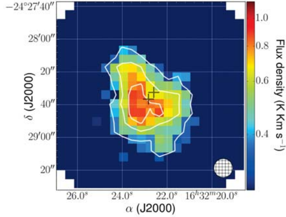
Figure 1. Moment 0 (integrated intensity) map of the J = 2 - 1 CN transition at 226.659 GHz. The white contours correspond to the emission of the same transition in steps of 0.2 \text{ K km s}^{-1} . The beam is shown at the bottom right of the figure. The crosses indicate the positions of sources A and B; the pointing direction of the pointed observations coincides with the position of source B to better than a fraction of an arcsecond.
