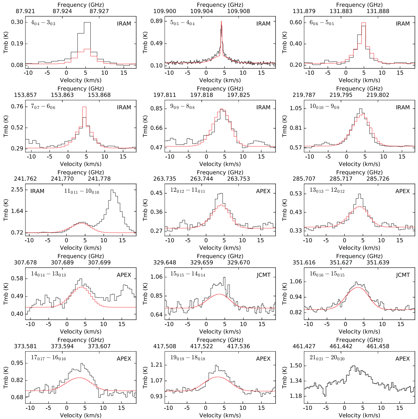
Figure B1. HNCO K_a = 0 transitions. The collision rate coefficient for the 21_{021} - 20_{020} transition was lacking and therefore it could not be modelled.
