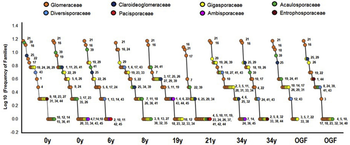
Fig. 3. Total frequency curves or Whittaker plots. The numbers represent the number of each species given in supplementary Table (S1). y = years in succession and OGF = old-growth forest.
