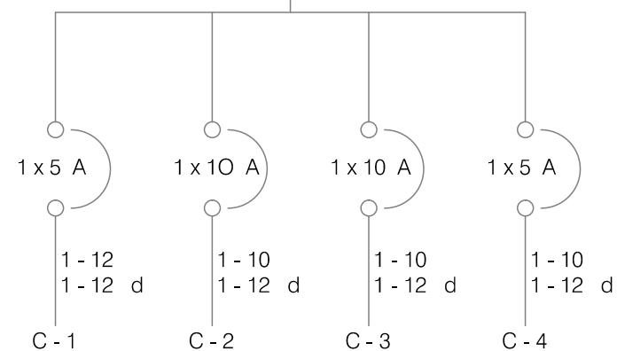
DIAGRAMA UNIFILAR
