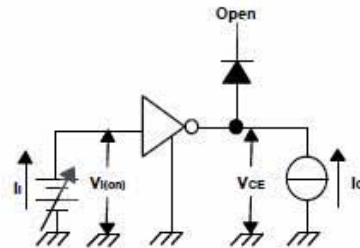
Fig.6 Vi(on) Test Circuit
