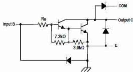
ULN2003A: R_B = 2.7k ULN2004A: R_B = 10.5k
