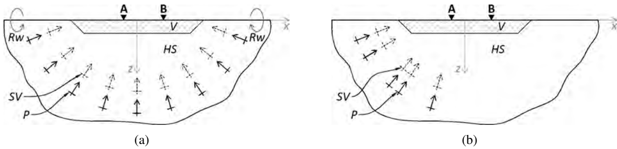
Figure A.3: Two types of excitations for the in-plane case: (a) Valley with isotropic illumination given by two sets of 200 plane P and SV waves each one ( \theta from \pi/2 to -\pi/2 , with respect to z axis), uniformly distributed and two Rayleigh waves from each side of the valley. (b) Valley with partial illumination of two sets of 50 plane P and SV waves each one, randomly distributed ( \theta from 0 to -\pi/2 , with respect to z axis). (The arrows distribution is only indicative). The same distributions were used for the anti-plane case but only using plane SH waves.
