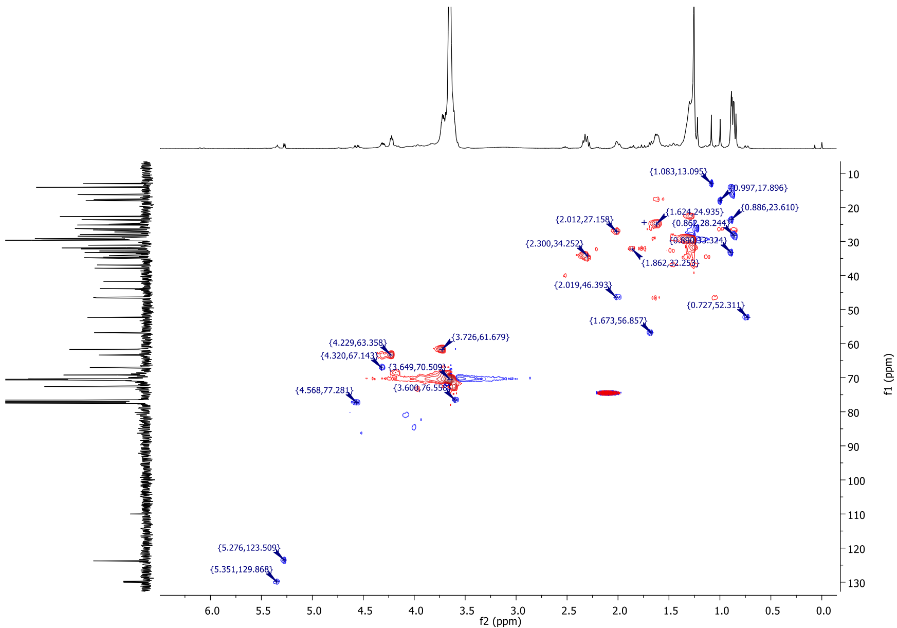
Espectro 19. HSQC ( \text{CDCl}_3 , 100 MHz) de 3\beta -palmitoiloxi- 1\beta,11\alpha -dihidroxi-olean-12-eno ( 93 )
