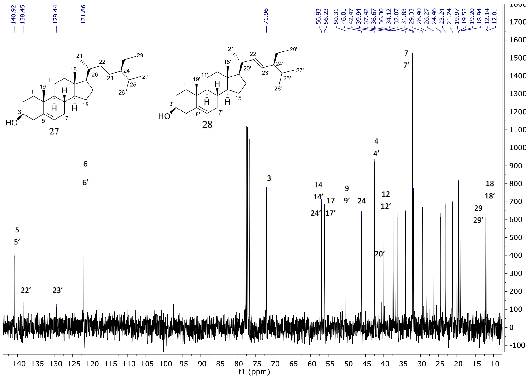
Espectro 10. RMN ^{13}\text{C} ( \text{CDCl}_3 , 75 MHz) de \beta -sitosterol ( 27 ) – estigmasterol ( 28 ) (4.3:1)
