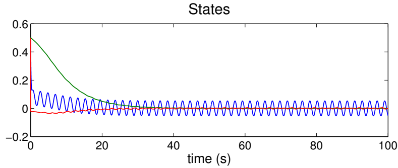
Figure 4.7: State trajectories of system (4.19) with the STA.
