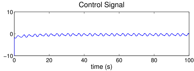
Figure 4.8: Super-Twisting Algorithm
