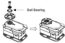
HN07-II (Bearing Set RX-28H)
