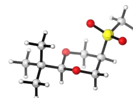
Cis-8
