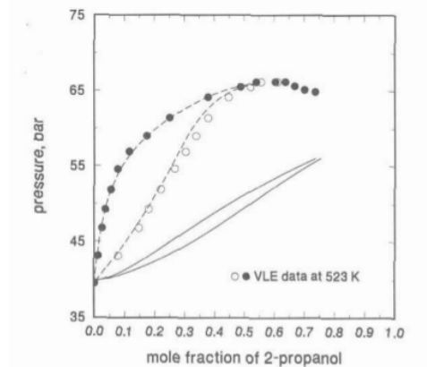
Figure 4.2.6. VLE correlation of the 2-propanol and water binary system at 523 K with the Huron–Vidal original (HVO) mixing rule combined with the NRTL excess free-energy model and the PRSV equation of state. The dashed lines represent results calculated with \alpha = 0.2893 and \tau_{12}/\tau_{21} = 0.3952/4.1518 obtained by fitting the experimental data, and the solid lines denote results calculated with \alpha = 0.2893 and \tau_{12}/\tau_{21} = 0.1019/1.2185 obtained from the DECHEMA Chemistry Series (Gmehling and Onken 1977, Vol. 1, Pt. 1, p. 325).
