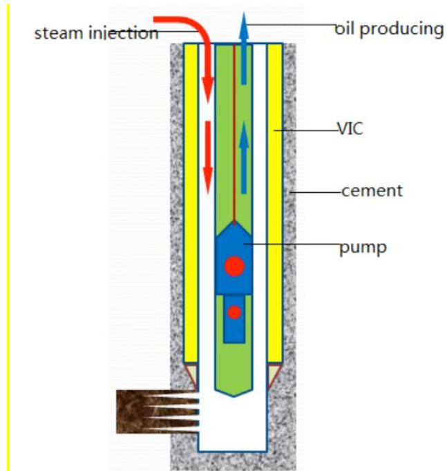
Fig.6 Schematic of VIC as part of Well completion
