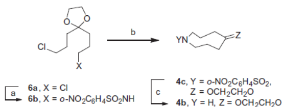
Scheme 3. An alternative preparation of 4b . Reagents and conditions: (a) o -NO 2 C 6 H 4 SO 2 NH 2 , n -Bu 4 NI, Na 2 CO 3 , MeCN/THF (1:1), Δ, 74%; (b) n -Bu 4 NI, n -Bu 4 NOH, dioxane, Δ, 55%; (c) C 6 H 5 SH, n -Bu 4 NOH, MeCN, 55–65%.
