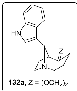
9-(1 H -indol-3-il)-1-azaespiro[bicyclo[4.2.1]nonano-5,2'-[1,3]dioxolano]
