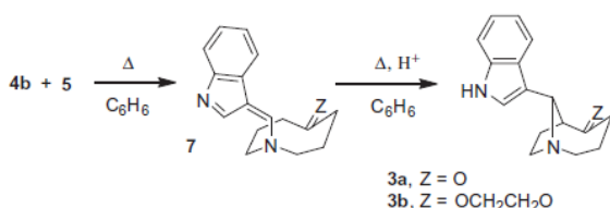
Scheme 4. Synthesis of the 9-(1H-indol-3-yl)-1-azabicyclo[4.2.1]nonane ring system.
