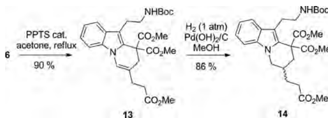
Scheme 3. Synthesis of pyridoindole 14 by alcohol removal.
