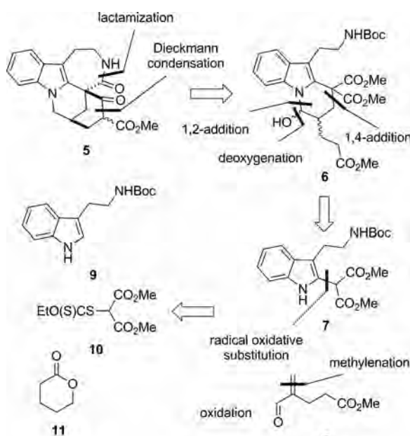
Scheme 1. Retrosynthetic plan for the preparation of pentacyclic intermediate 5 .
