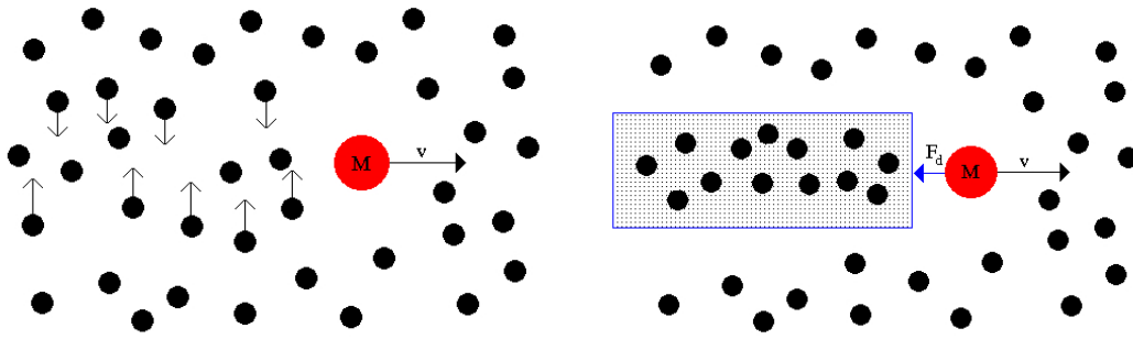
FIGURE 1.7: Dynamical friction simplified sketch. Schombert Lectures.
