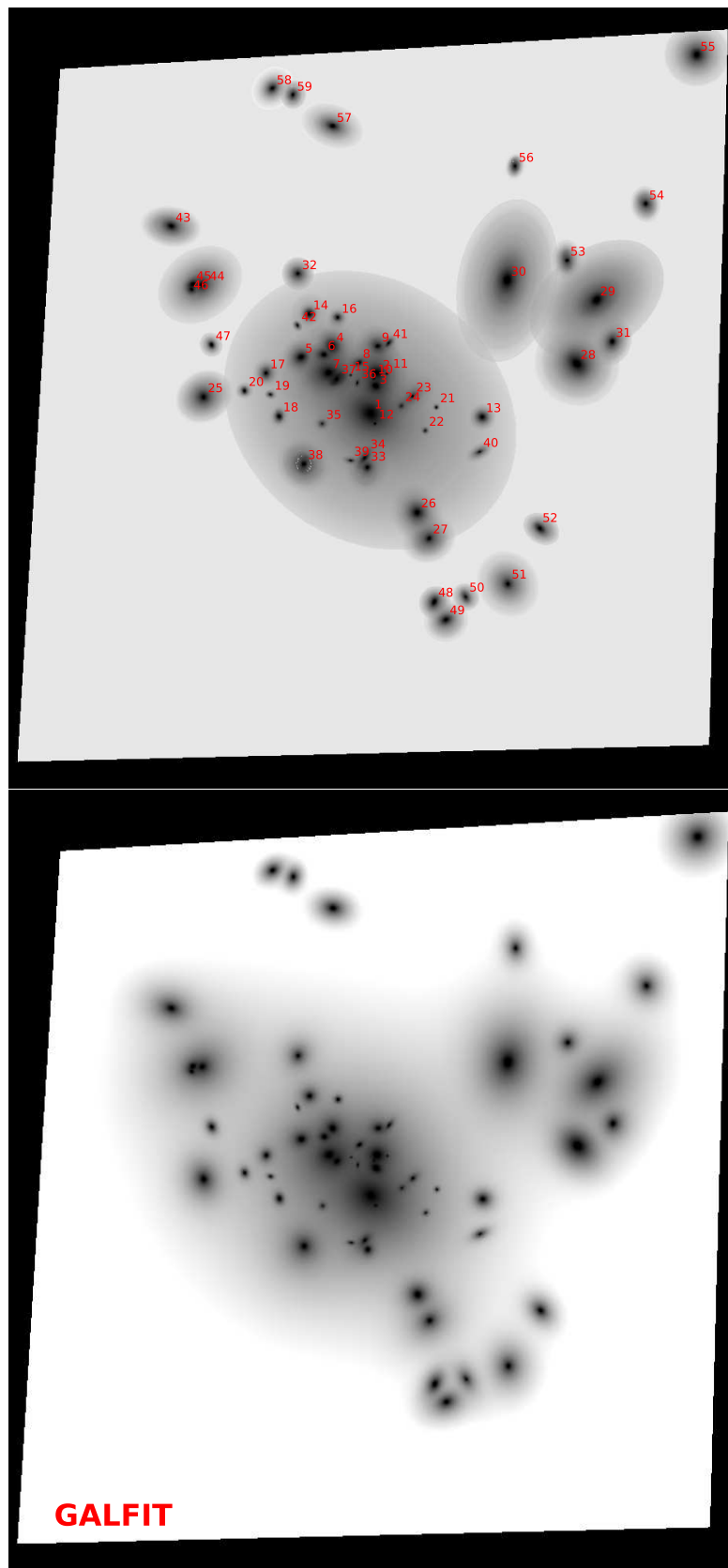
FIGURE 4.16: The 59 brightest galaxies within A1689. Top: bmodels constructed with ellipse/IRAF. Bottom: Sérsic models constructed with GALFIT.
