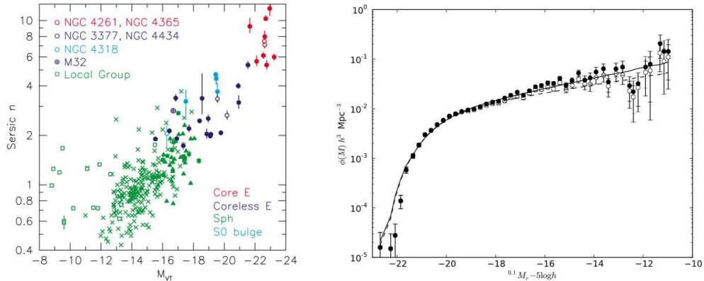
FIGURE 2.3: Left panel: Sérsic index, n , vs. visual absolute magnitude. Kormendy et al. (2009). Right panel: Luminosity function for galaxies with z < 0.1 from the Galaxy and Mass Assembly survey (dots); the solid line shows the best Schechter function. Loveday et al. (2012).
