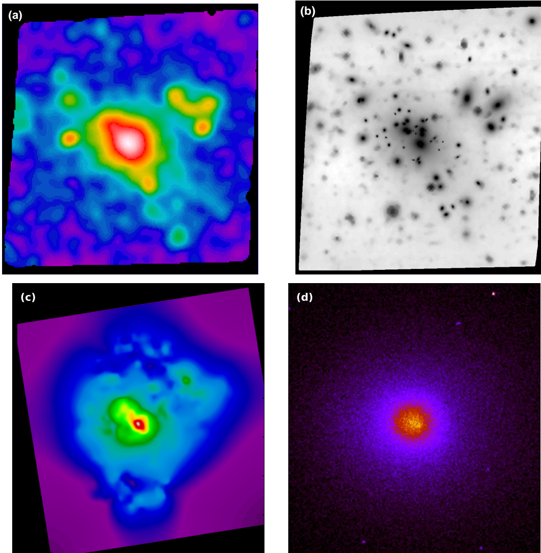
FIGURE 4.12: (a) Surface number density of GC candidates, smoothed with a Gaussian with \text{FWHM} = 10'' (300 pix); (b) surface brightness distribution from isophotal models of 59 galaxies plus the SExtractor background map; (c) lensing-derived total surface mass density (includes baryonic and non-baryonic components); (d) X-ray surface brightness distribution (from Chandra archive).
