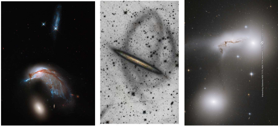
FIGURE 2.6: Left panel: Arp 142; credit: NASA, ESA, and the Hubble Heritage Team (STScI/AURA). Middle panel: NGC 5907, Martínez-Delgado et al.(2008). Right panel: Hickson Compact Group 90; credit: NASA, ESA, and R. Sharples (University of Durham).
