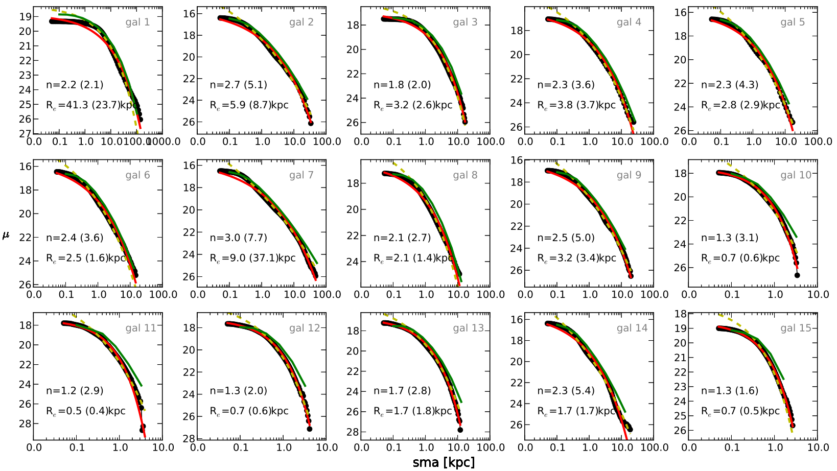
FIGURE 4.17: Surface brightness profiles of the brightest 59 galaxies in A1689 (black dots). The curves show the best Sérsic fit in 1D (red), GALFIT Sérsic 2D fit (yellow dashed), and \mu_{SB} in ellipsoidal annuli from the GALFIT models (green). The corresponding n and R_e from the 1D fitting and GALFIT models (in parenthesis) are indicated.
