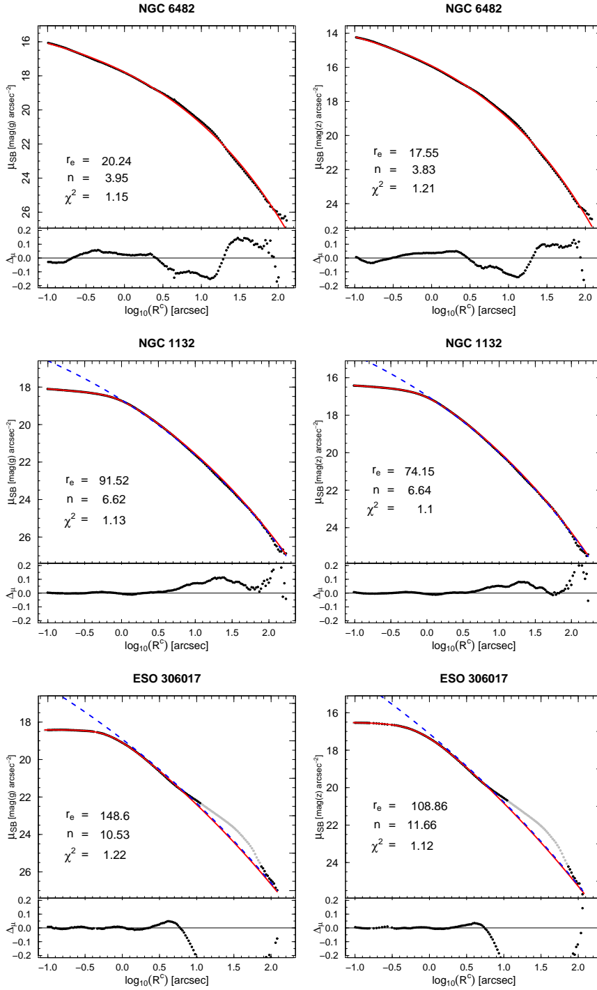
FIGURE 3.7: Galaxy surface brightness distribution as a function of the isophotal equivalent circular radius R^c . Left panels: g -band. Right panels: z -band. Dots: data after subtraction of the fitted sky value. Solid red lines: best fit profiles: single Sérsic for NGC 6482, and core-Sérsic for NGC 1132 and ESO 306-G017 (gray dots were not included in the fits of this galaxy). Dashed blue lines: single Sérsic for NGC 1132 and ESO 306-G017. Fit residuals are shown in the bottom of each panel.
