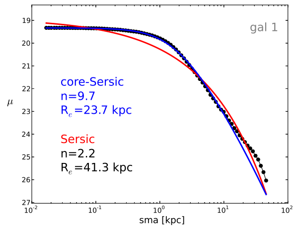
FIGURE 4.18: Surface brightness radial profile of the BCG in A1689 (black dots). The curves show the best single Sérsic fit (red) and the best core-Sérsic fit (blue).
