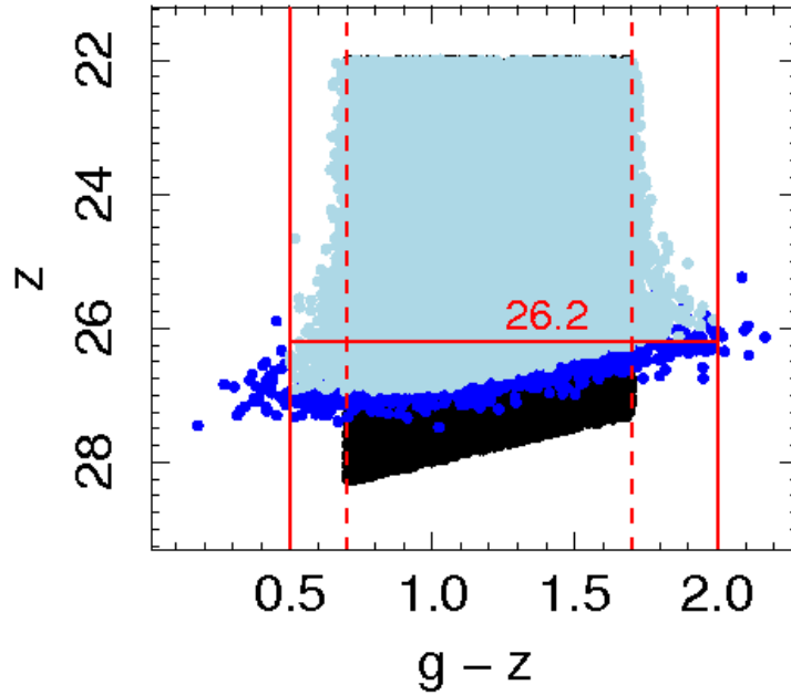
FIGURE 3.10: Color magnitude diagram of added stars. The black points are the constructed stars (input values), overplotted are all the recovered objects (dark blue points) and the recovered objects after applying the same constraints as for GC selection for ESO 306-G017 (light blue points).
