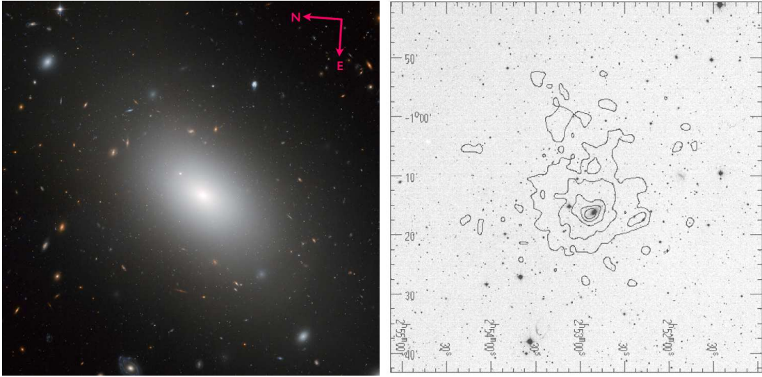
FIGURE 3.4: Fossil group NGC 1132. Left: optical ACS/HST RGB image, \text{FOV} \sim 3'3 \times 3'3 . Right: optical DSS image with ASCA X-ray contours of the diffuse emission, \text{FOV} 1^\circ \times 1^\circ (Mulchaey & Zabludoff 1999).
