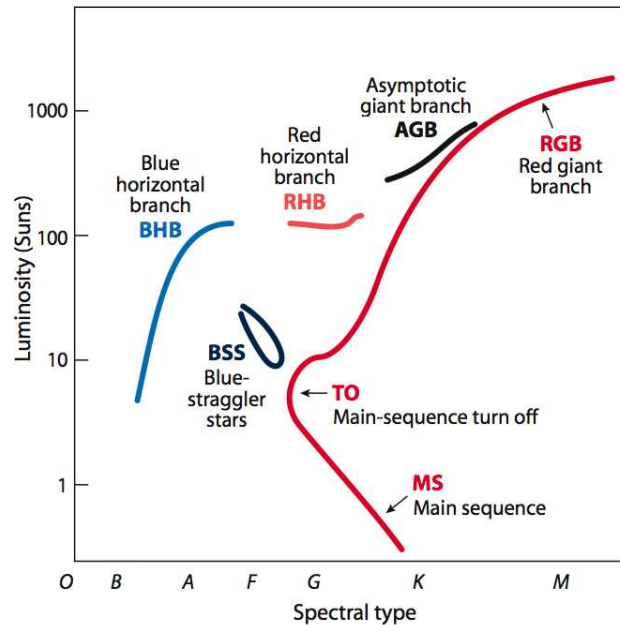
FIGURE 1.4: Representation of a GC CMD, showing the main evolutive stellar stages. Djorgovski (1998).
