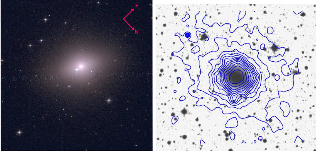
FIGURE 3.3: Fossil group NGC 6482. Left: optical ACS/HST RGB image, \text{FOV} \sim 3'.3 \times 3'.3 . Right: optical DSS image with Chandra X-ray contours of the diffuse emission, \text{FOV} 8' \times 8' (Khosroshahi et al. 2004).
