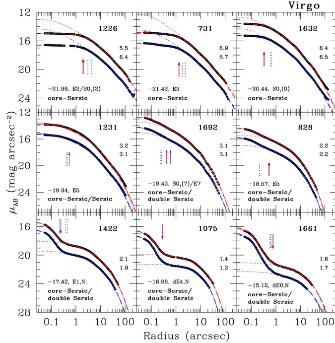
FIGURE 2.2: Surface brightness profiles in the g and z ACS/WFC filters for 9 representative Virgo cluster galaxies. Côté et al. (2007).
