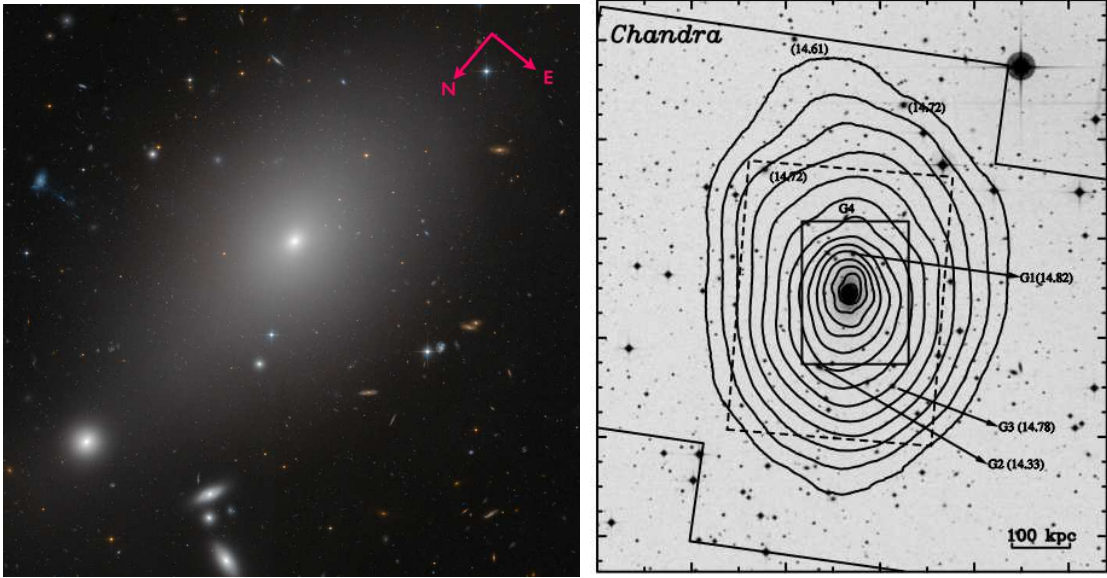
FIGURE 3.5: Fossil group ESO 306-G017. Left: optical ACS/HST RGB image, \text{FOV} \sim 3'3 \times 3'3 . Right: optical DSS image with Chandra X-ray contours of the diffuse emission, \text{FOV} \sim 19' \times 22' (Sun et al. 2004).
