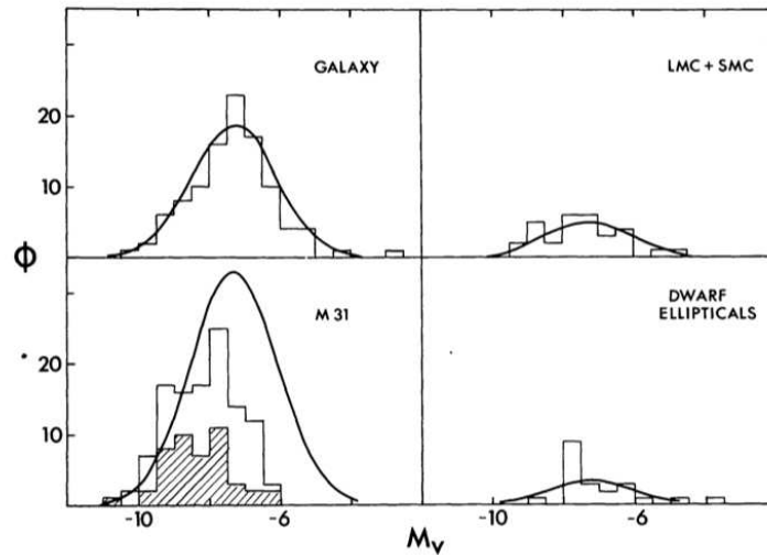
FIGURE 1.14: GC luminosity distributions for Local Group galaxies (histograms). \Phi(M) is the number of GCs in intervals of 0.5 mag. The solid curves are scaled Gaussians with M_V^0 = -7.3 and \sigma_{\text{GCLF},V} = 1.2 . Harris & Racine (1979).
