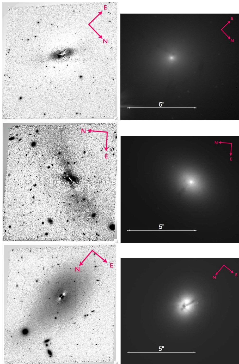
FIGURE 3.8: Left: residual z -band images after subtracting the best single Sérsic model. Right: Inner regions of g -band images; dust is present in all cases. Top to bottom: NGC 6482, NGC 1132, and ESO 306-G017.
