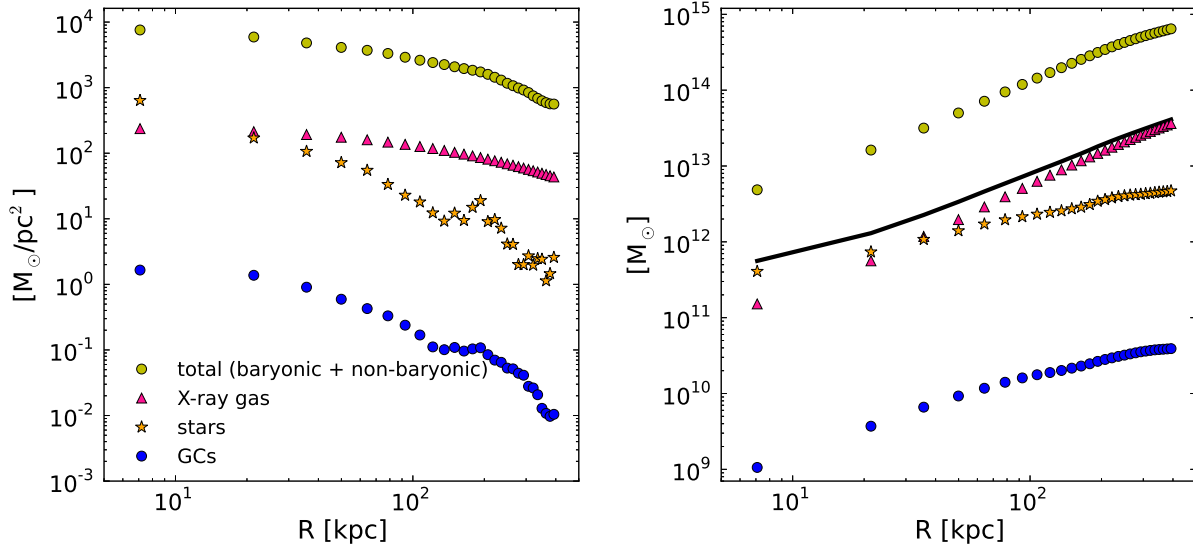
FIGURE 4.14: Left panel : radial mass density profile for each component. Right panel : cumulative mass profiles versus radius. The thick black line indicates the cumulative profile of the baryonic mass, \mathcal{M}_{\text{baryon}} = \mathcal{M}_{\text{Xray}} + \mathcal{M}_{\star} .
