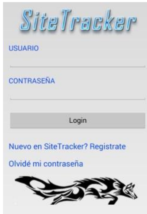
Figura 5.6. activity_main.xml
