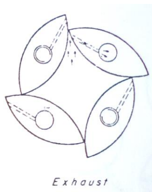
Figura 2.6 Escape axial (Chicurel, DEVELOPMENT OF A NOVEL ENGINE, 1979) (Chicurel, Rotary expander for operation with waste or solar derived heat, 2011)
