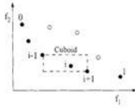
Fig. 1. Crowding-distance calculation. Points marked in filled circles are solutions of the same nondominated front.
