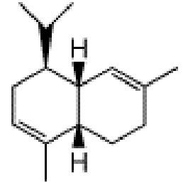
\alpha -Mouroleno 38
