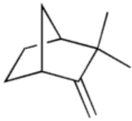
Canfeno 13
