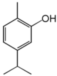
Carvacrol 14
