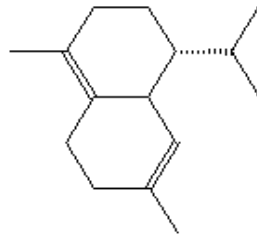
\alpha -Cubeneno 34
