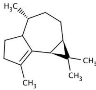
\alpha -Gurjuneno 37
