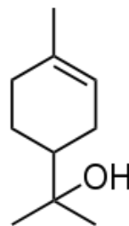
\alpha Terpineol 24
