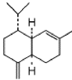
\gamma -Mouroleno 39
