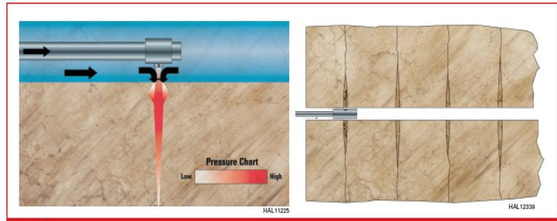
Fig. 6 - In the SurgiFrac process, sand-laden fluid pumped through a Hydra-Jet™ tool impinges on the formation creating a cavity. As the cavity is formed, pressure on the bottom of the cavity increases, eventually initiating a fracture. Annular fluid is pulled into the fracture, helping to extend it.
