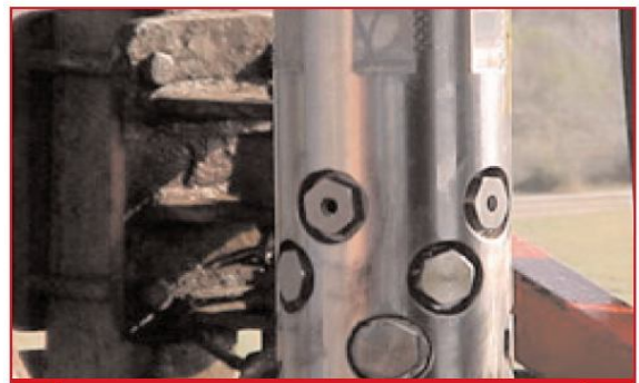
Fig. 8 – SurgiFrac SM service uses a specially designed high-pressure hydrajetting tool similar to those commonly used in oilfield applications to abrade, penetrate, or cut steel casings or rock formations. The tool can be designed to meet well conditions.
