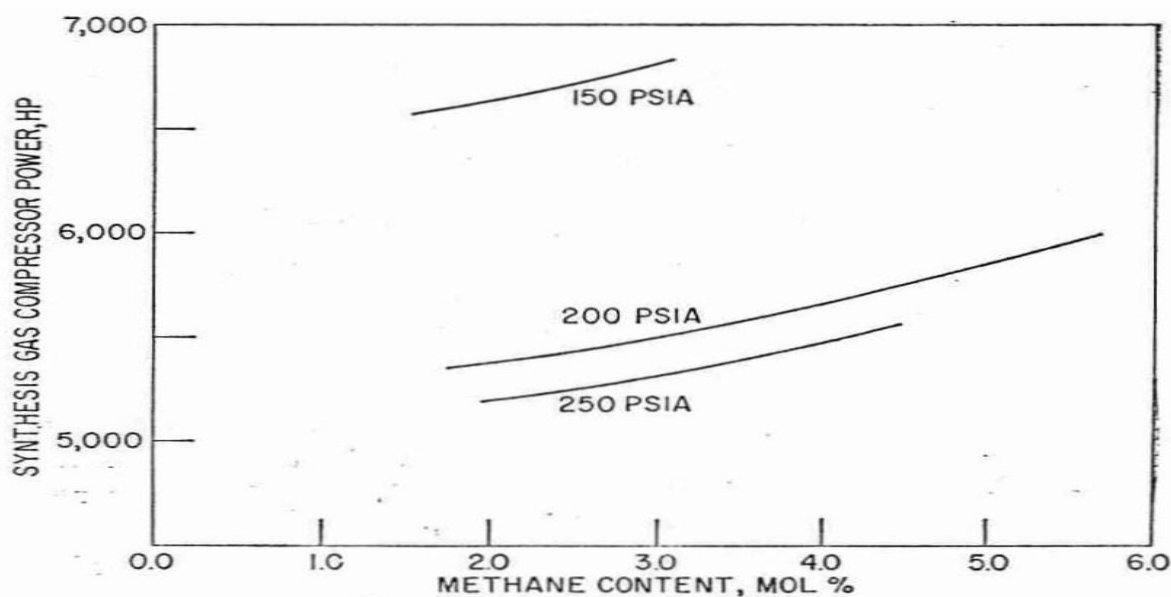
Fig. 4—Typical synthesis gas compressor horse power versus methane content for 500 STD methanol plant.
