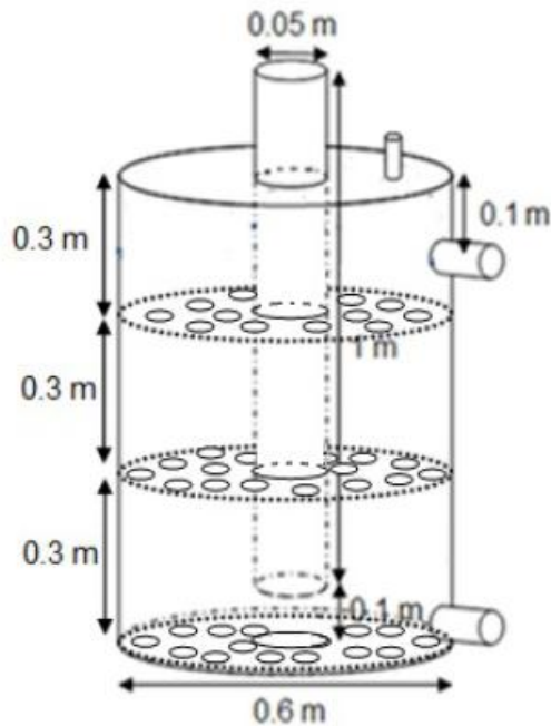
Figure 3.13: Volumen de control completo
