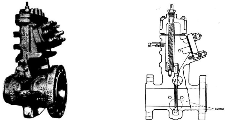
Figura 8.11. Fitting
