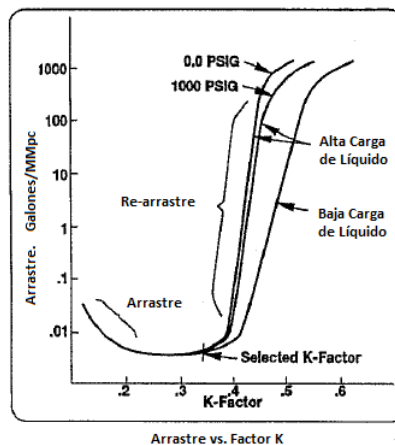
Figura 4.6. Arrastre vs. Factor K
