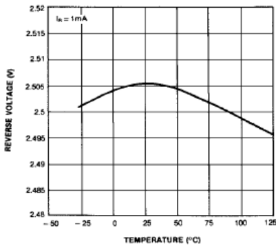
Figure 3. Temperature Drift
