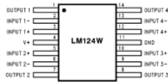
See NS Package Number W14B or WG14A
