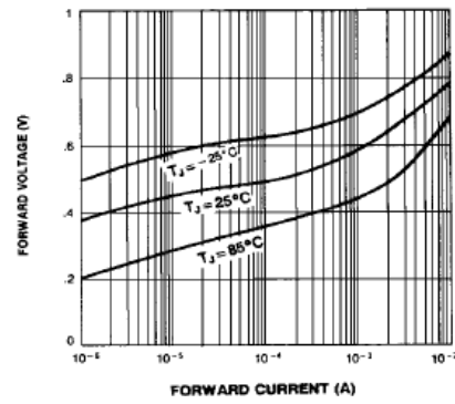
Figure 4. Forward Characteristics
