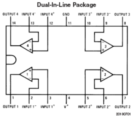
Top View See NS Package Number J14A
