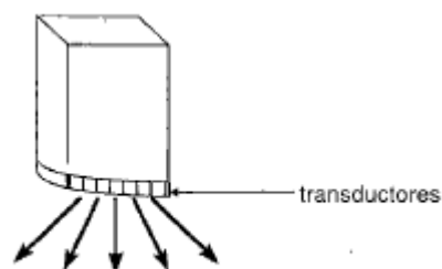
Figura 1.14 Transductor sectorial
