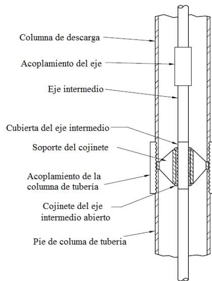
Figura 2.3 Ensamble de la columna [nationalpumpcompany, 2005] 11
